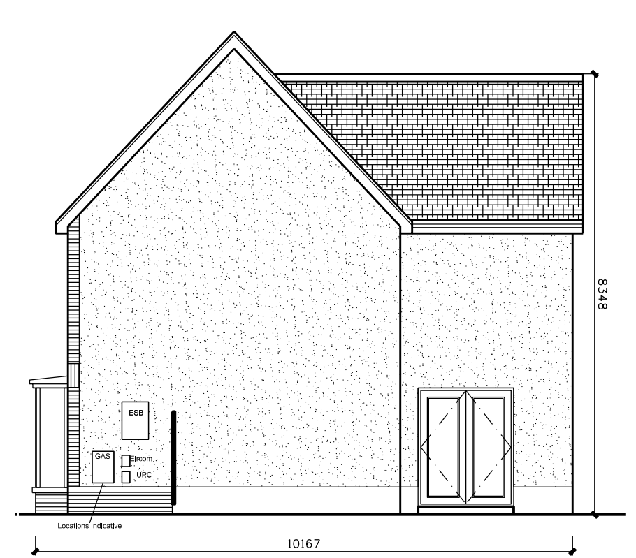
SIDE ELEVATION 2
