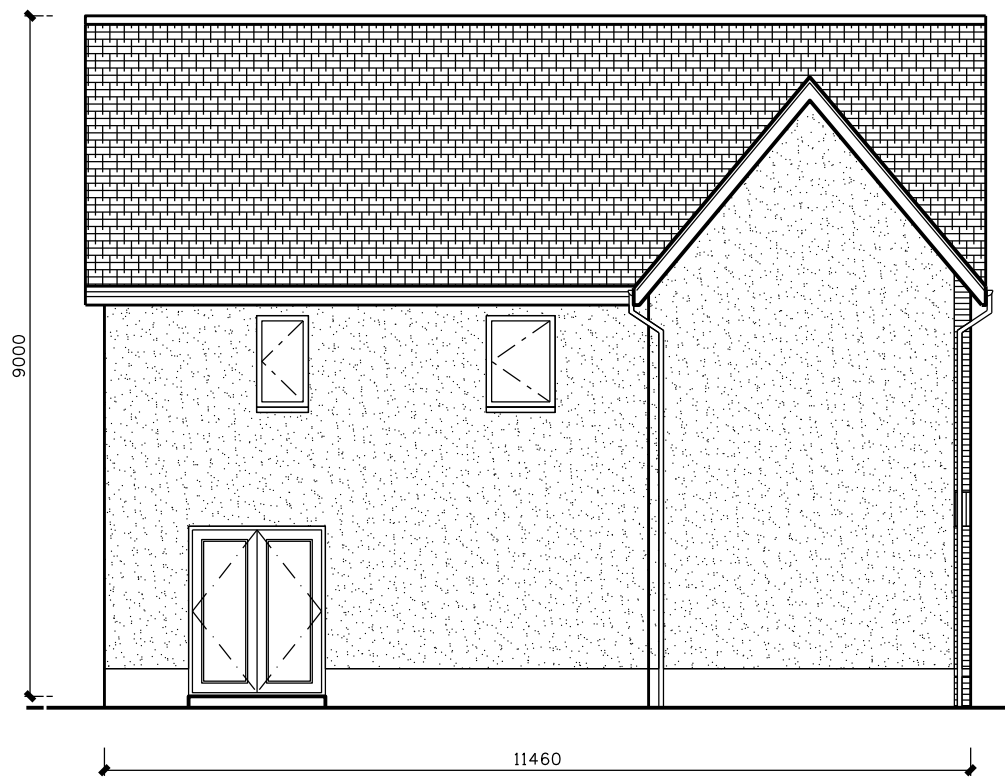
REAR ELEVATION
